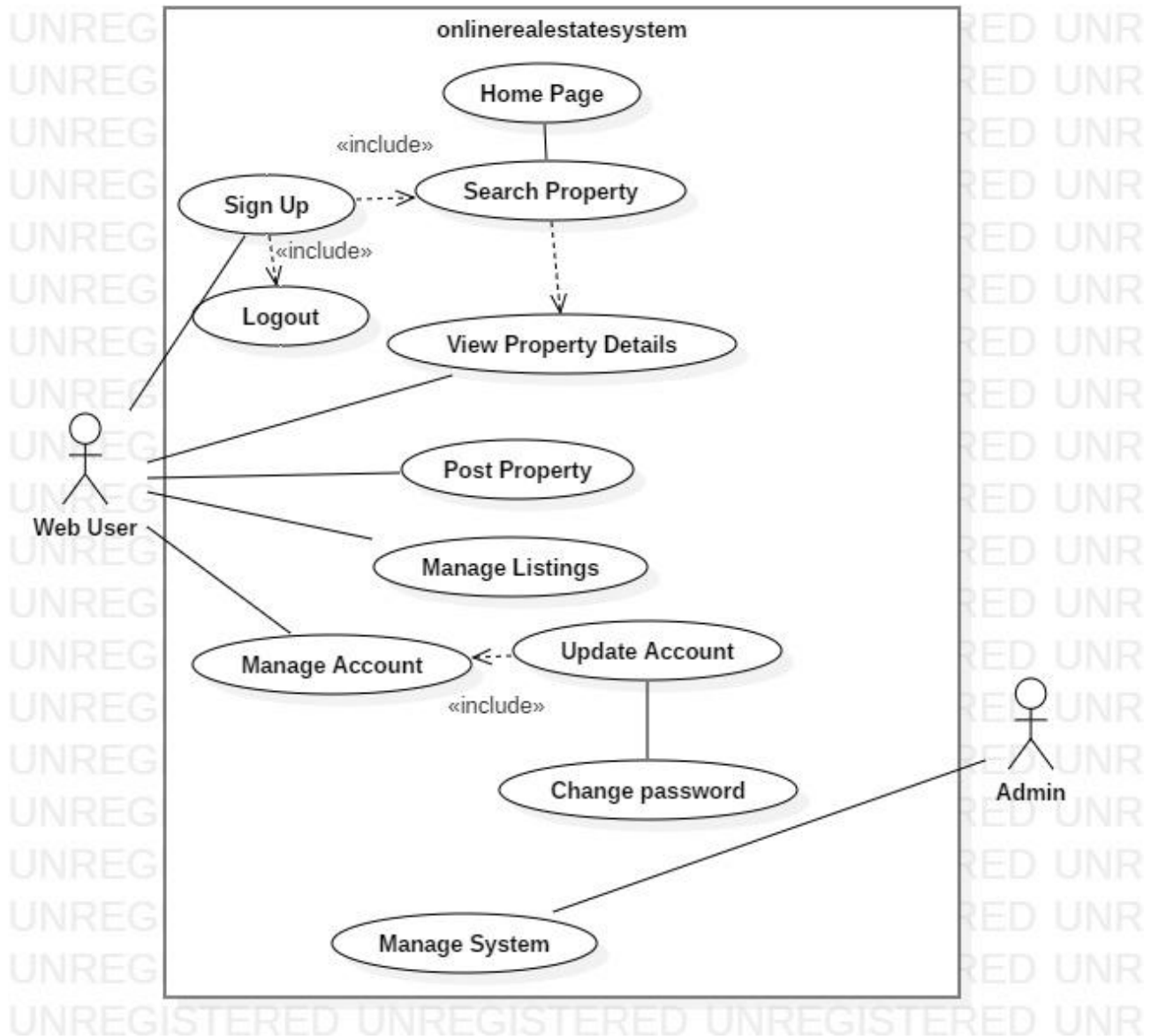
FIGURE 6: Web User Use Case Diagram
