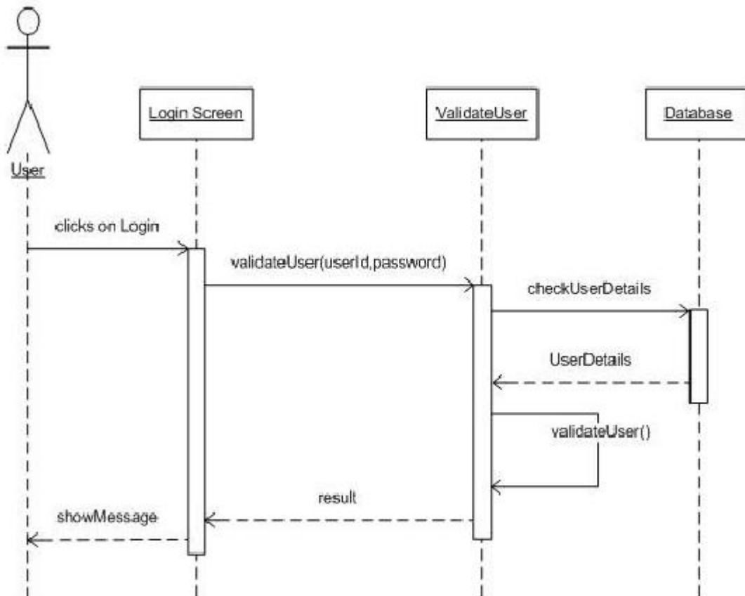
FIGURE 8: Sequence Diagram of User Login
