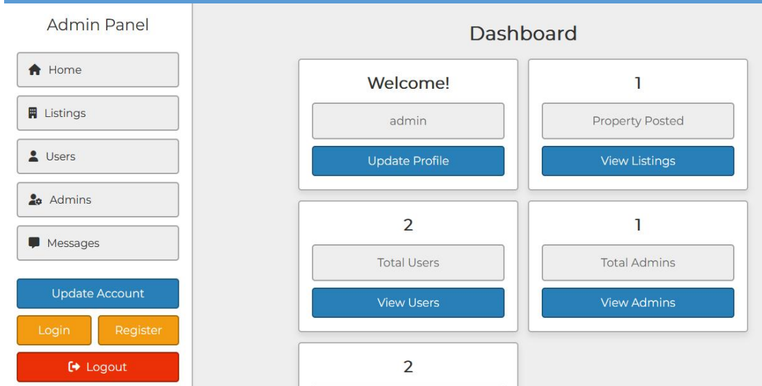
FIGURE 14: Admin Page
